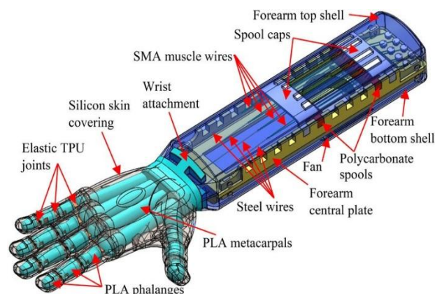
Diag.1. Model of the transradial prosthetic arm.
